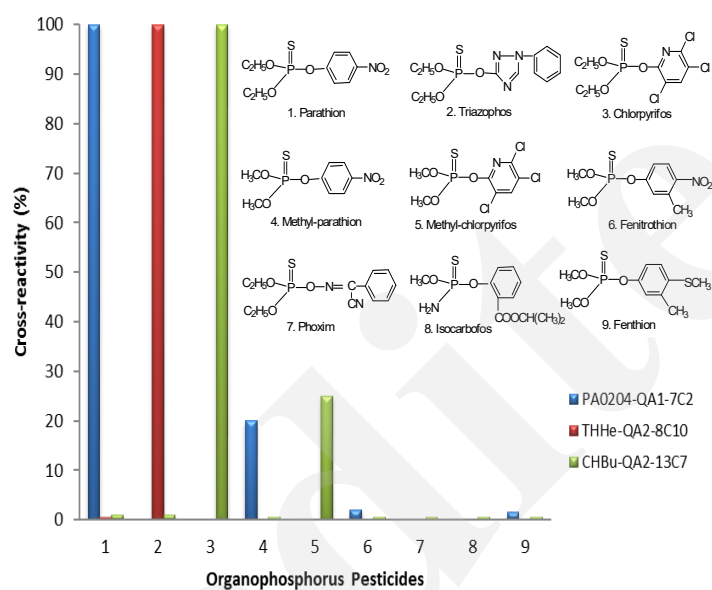
Fig. 4 Cross-reactivity study of three new mAbs to some organophosphorus pesticides
